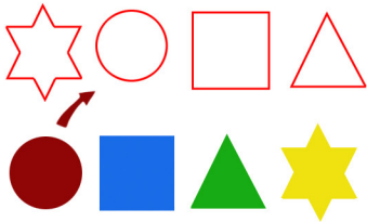
Sort Shapes
